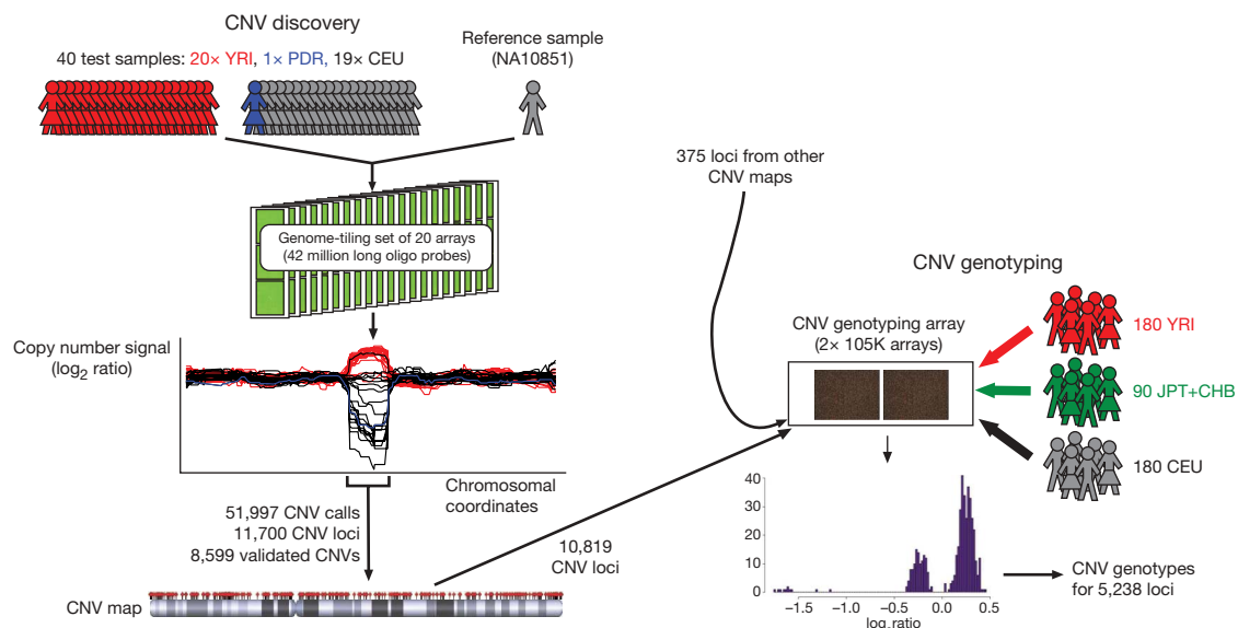
Figure 1 | Overview of experimental strategy for CNV discovery and genotyping. Overview of the discovery and genotyping phases of this project, with the former generating a new map of CNV locations and the
