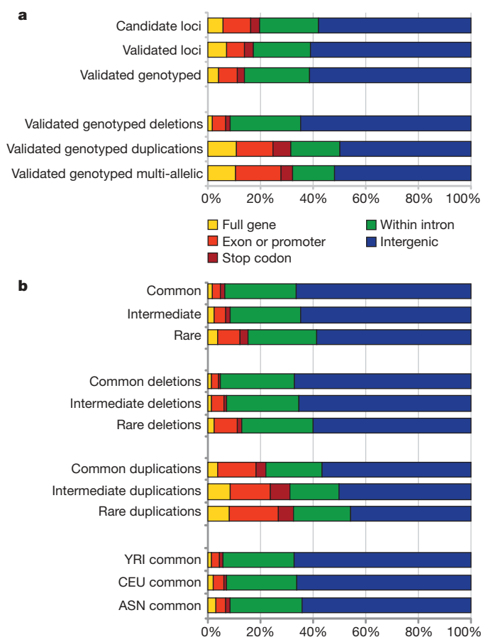
Figure 2 | Functional impact of CNVs by type, frequency and population. a , Impact on genes of sets of CNV at different stages of characterization (candidate, validated, genotyped/ genotyped loci). Genotyped CNVs are split into different classes (deletion, duplication and multiallelic). b , Impact on genes of CNV classes based on population frequency. Frequency classes: common (MAF \geq 0.1 in any population), intermediate (0.1 > MAF > 0.01), rare (MAF \leq 0.01 in all populations). ASN denotes JPT+CHB.
